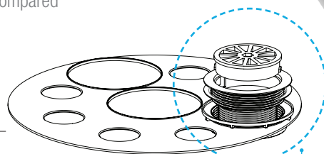
Shower base waste with self-supporting disc
