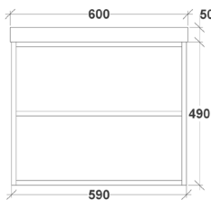
FRONT VIEW 50mm
