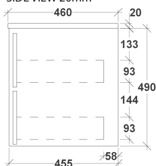
SIDE VIEW 20mm
