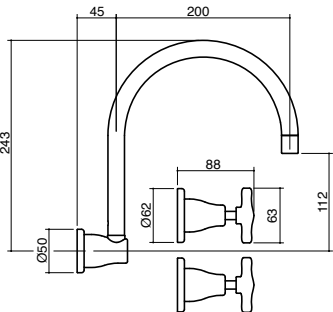
15 Cross Wall Sink Set
