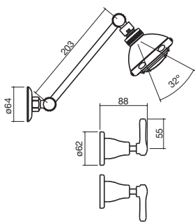
4 Deluxe Lever Shower Set
