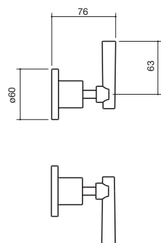
4 Wall Top Assembly
