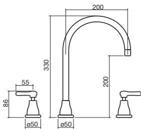
1 Lever Hob Bath/Spa Set
