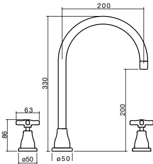
11 Cross Hob Bath/Spa Set
