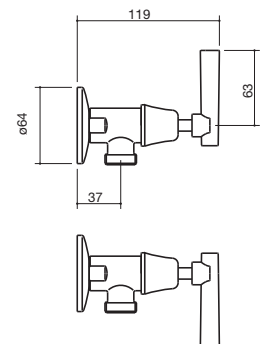
6 Washing Machine Stops
