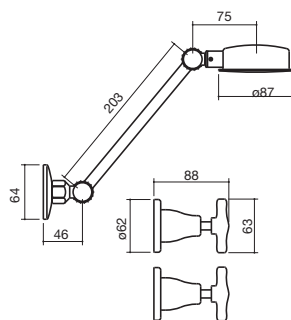
8 Standard Cross Shower Set
