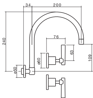
3 Wall Sink/Laundry Set
