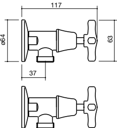
13 Cross Washing Machine Stops
