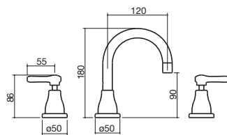
5 Lever Basin Set
