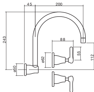
2 Lever Wall Sink Set
