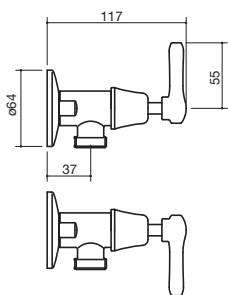
7 Lever Washing Machine Stops
