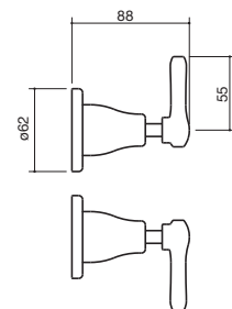
6 Lever Wall Top Assembly
