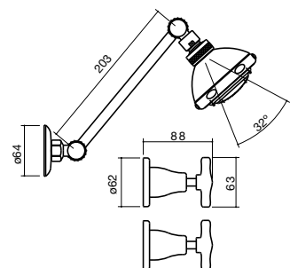
9 Deluxe Cross Shower Set
