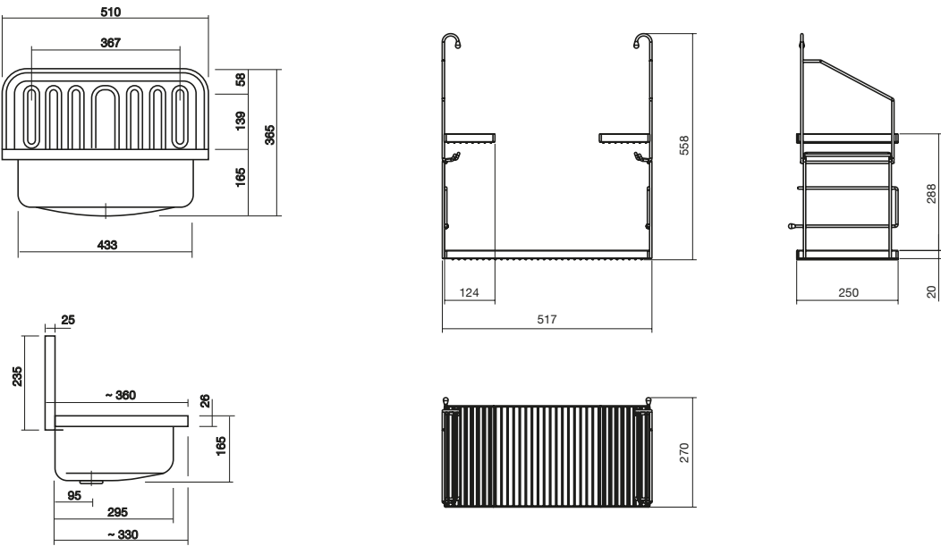
Klassiker Wall Basin No taphole 9501358 Utensilo Steel Shelf 1810642
