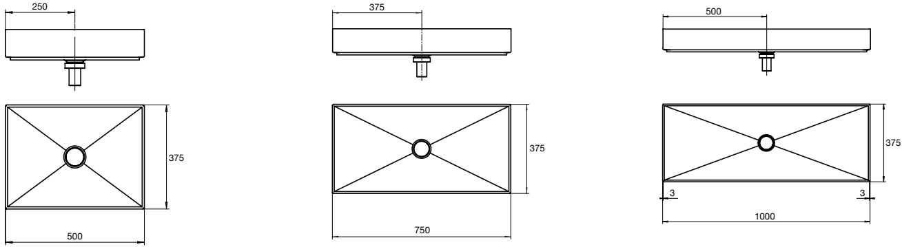
Metaphor 500 Counter Basin No taphole 9502483
