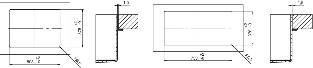
Metaphor 500 Flush Mounted Basin No taphole 9506197
