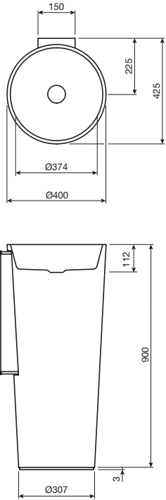
Scpio 400 Washstand No taphole 9508138
