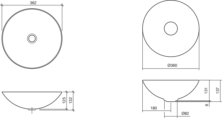
Circa 360 Vessel Basin 1805858 Also available: Gloss Black 9502827 Matte Black 9506244 Bi-Colour 9508143 Dark Iron 9508142 Circa Terra 360 Vessel Basin Gravel Matt 1806078 Nordic Matt 1806079 Oyster Matt 1806080
