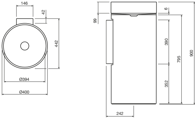
Unisono 400 Freestanding Basin Bi-Colour, No taphole 9508140
