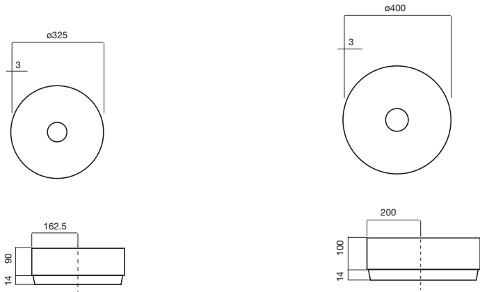
Unisono Counter Basin 325 No taphole 9503961
