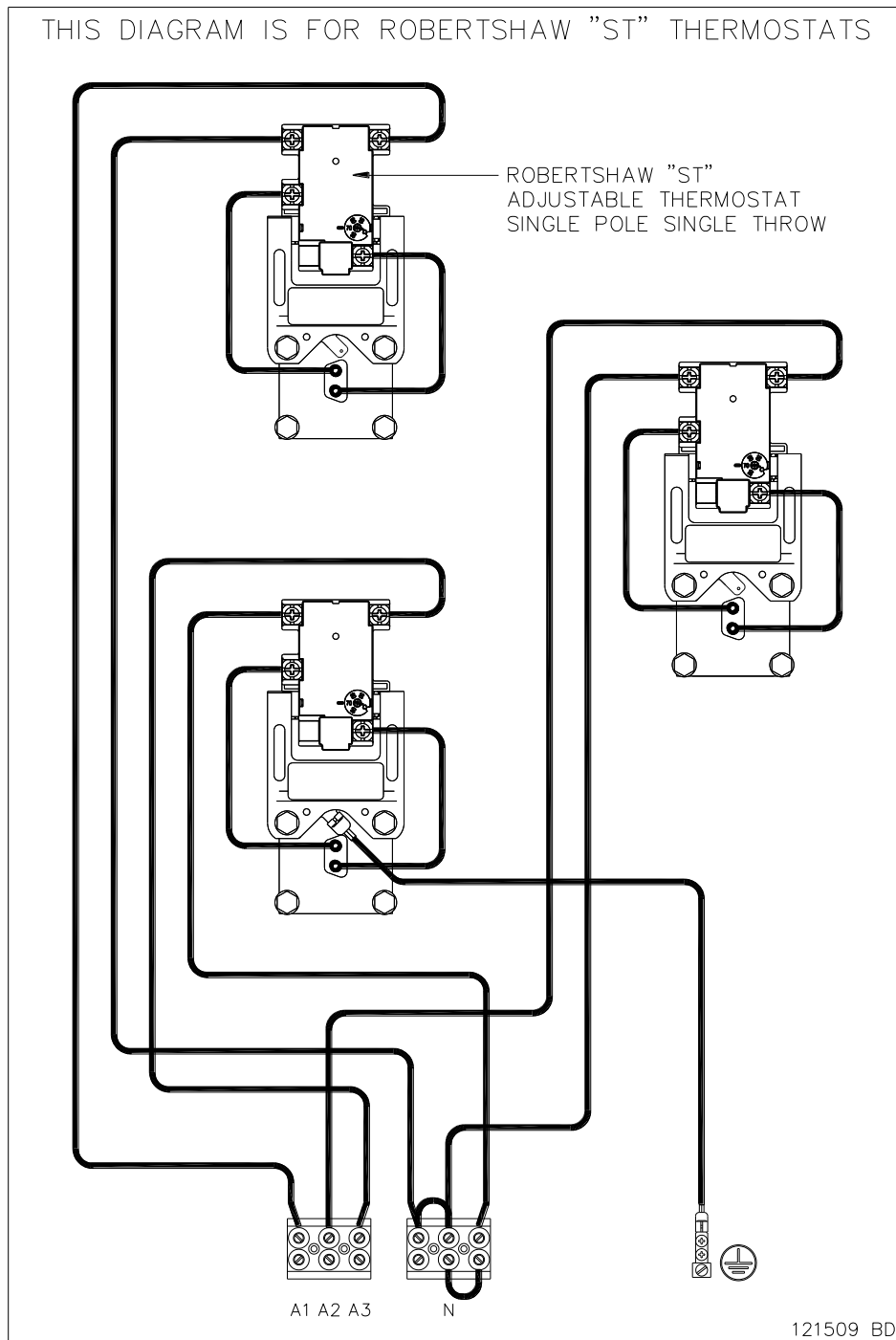
Electrical Circuit for 623 Models – Robertshaw "ST" Thermostats
