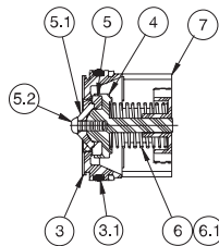
Check Assembly
