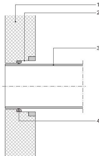
Figure 23: Connection with prefabricated duct connector
