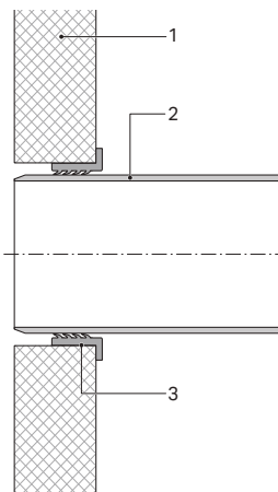
Figure 24: Connection with sealing of connection
