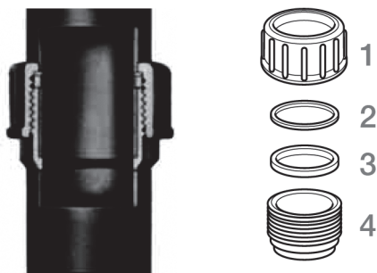
Figure 33: Screw-threaded joint without flange bushing (available ø 40–110 mm)
