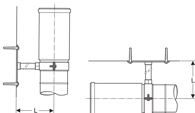
Figure 5: Anchor bracket
