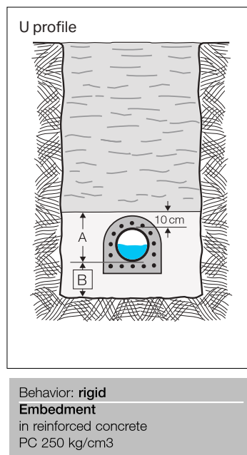
Figure 17: U profile
