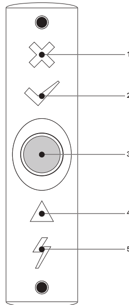
Figure 29: Operating interfaces of the electrofusion machine
