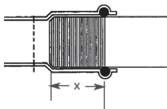
Figure 32: Ring seal socket joint (available ø 40 - 160 mm)
