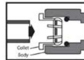
To connect, push tube through collet ring into body.
