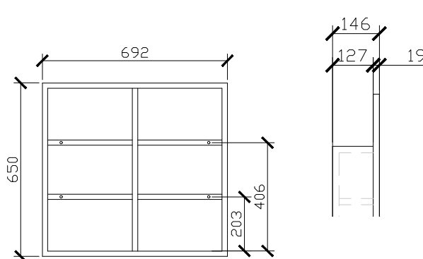
SIDE VIEW for all sizes
