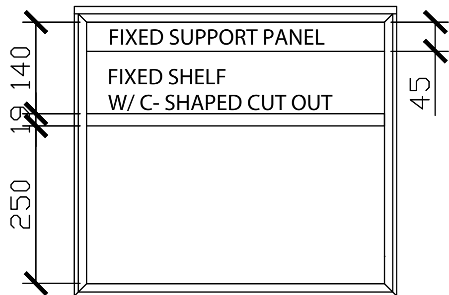
INTERNAL VIEW
