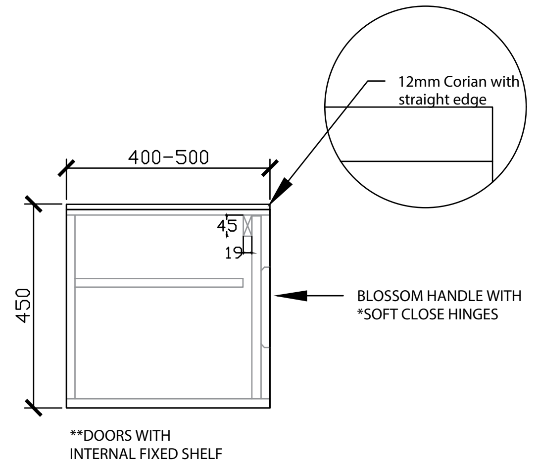
SIDE VIEW
