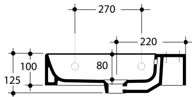
Cento Mini Counter/Wall Basin 450 x 250mm - 1 Taphole
