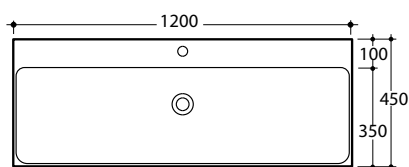
Cento Counter/Wall Basin 1200 x 450mm - 1 Taphole
