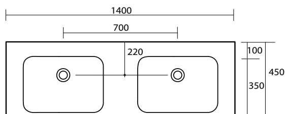
Cento Counter/Wall Basin 1400 x 450mm - 0 Taphole
