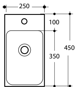
Cento Mini Counter/Wall Basin 250 x 450mm (Rear) - 1 Taphole
