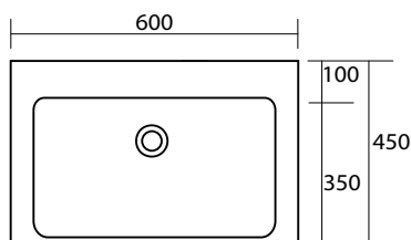
Cento Counter/Wall Basin 600 x 450mm - 0 Taphole
