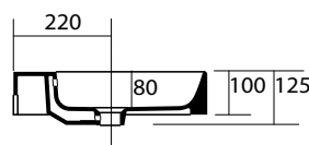
Cento Counter/Wall Basin 600 x 450mm - 0 Taphole
