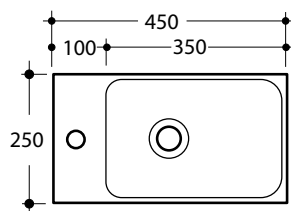
Cento Mini Counter/Wall Basin 450 x 250mm - 1 Taphole
