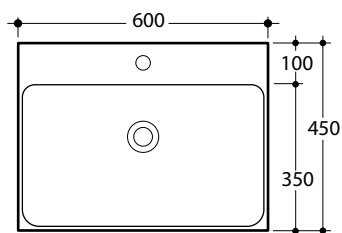
Cento Counter/Wall Basin 600 x 450mm - 1 Taphole
