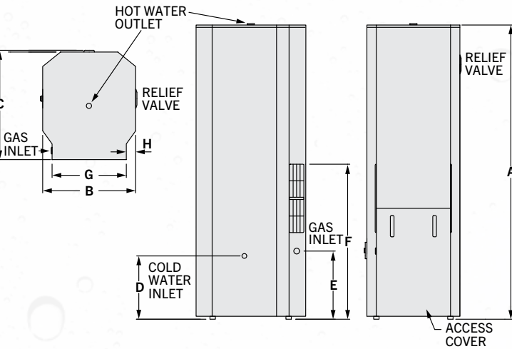
RHEEM 340 GAS SS
