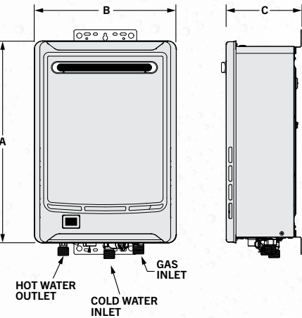
RHEEM CONTINUOUS FLOW 12 - 26L
