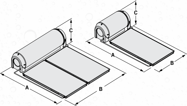
RHEEM PREMIER® HILINE SOLAR HOT WATER HEATER
