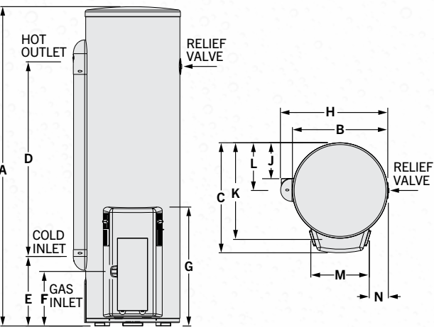
RHEEM 4 STAR / 5 STAR / STELLAR / INDOOR
