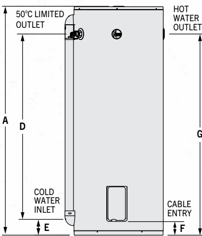
RHEEM DUALTEMP 125L & 250L
