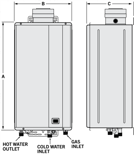
RHEEM ULTRA 28L (Internal)
