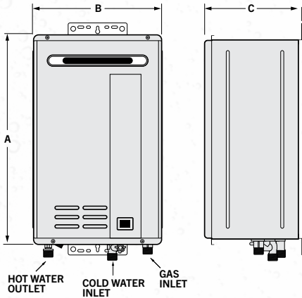
RHEEM ULTRA 28L (External)
