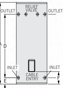
RHEEM ELECTRIC 25L - 125L
