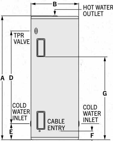
RHEEM ELECTRIC STAINLESS STEEL 80L - 315L
