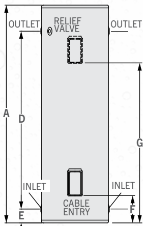
RHEEM ELECTRIC 160L - 400L
