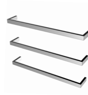
●● Bloc Single Heated Towel Rail 630mm, 830mm Stainless Steel (grade 304) Polished Stainless Steel and Matte Black Hardwired Projection: 100mm Sold individually and transformer sold separately
