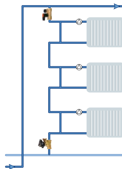
1-pipe system
