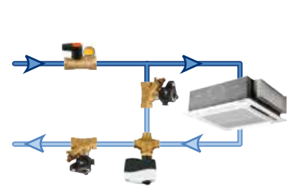
Fan coil unit application.
