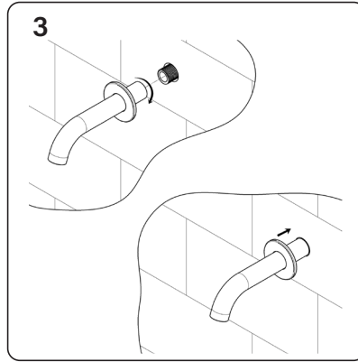
Install Flange & Spout
