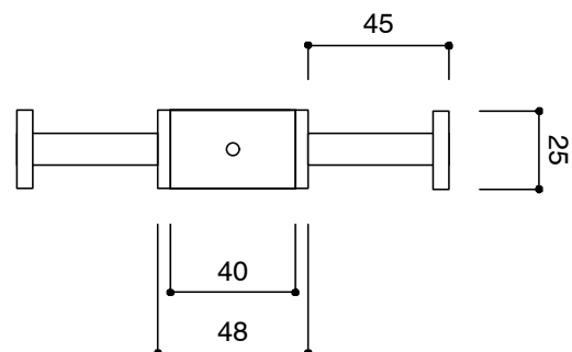
TUBE HOOK FRONT
