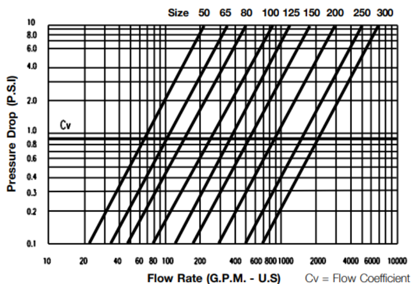
FLOW CHARACTERISTICS CHART
