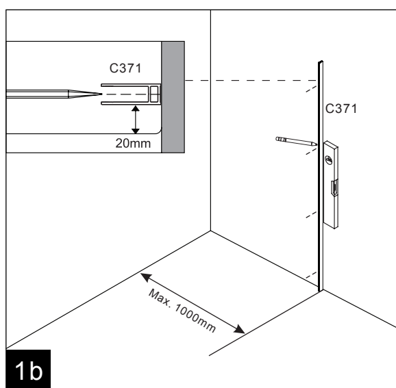
b- Shower screen installed with tiled floor
