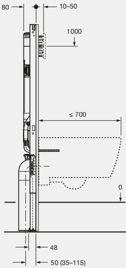
Sigma Wall hung install
