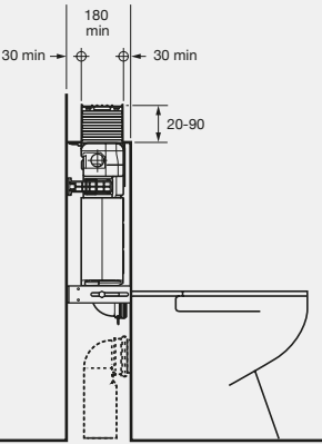
Omega Undercounter Cistern Back to wall
