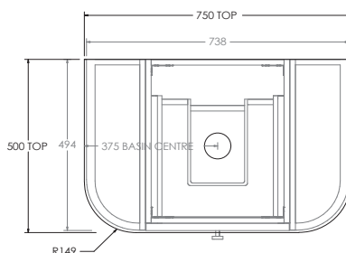
Top View Centre
