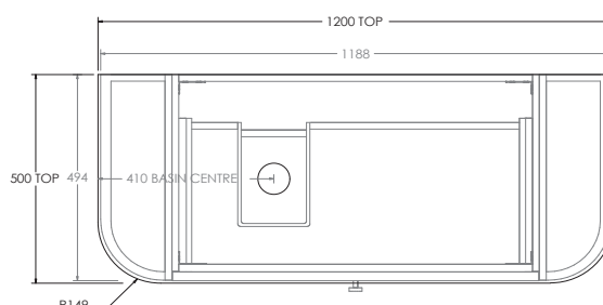
Top View Offset (Left or Right)
