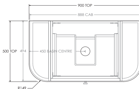
Top View Centre
