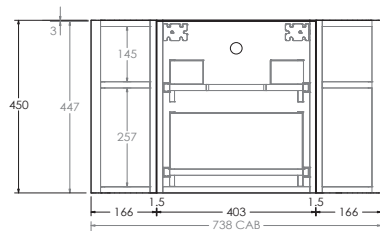
900mm Front View
