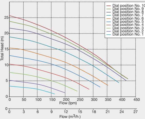
Hydraulic Performance - H400VSPBT
