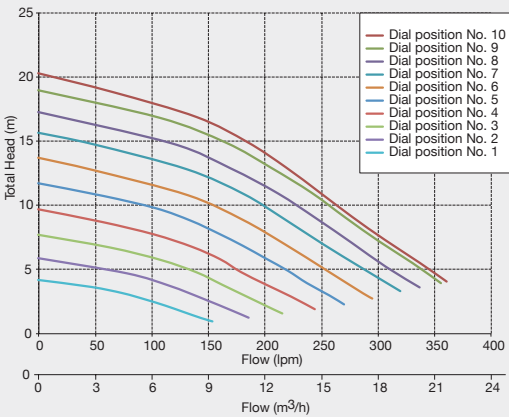
Hydraulic Performance - H280VSPBT
