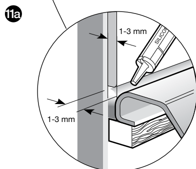
Built-in
