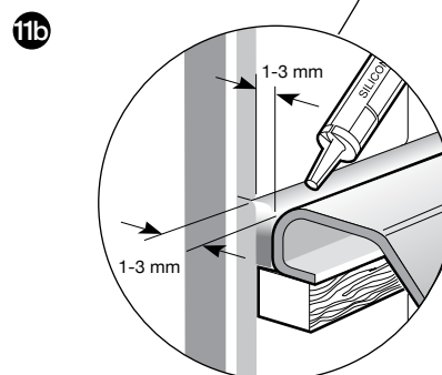
Flush-mounted
